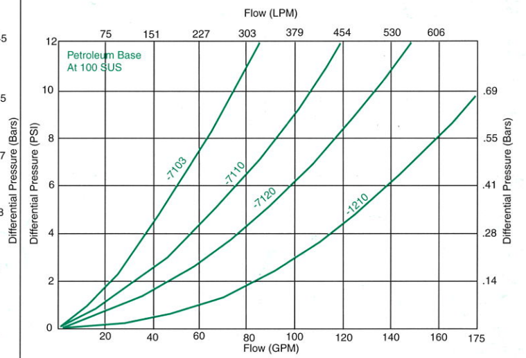
Graph 4. Typical Pressure Drop Versus Flow: Double Length Assembly 269321-0000/5 & 67366-Media Part Number (See Below)
