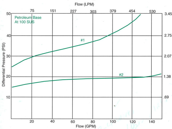
Graph 3. Typical Pressure Drop Versus Flow: Extended Length Assembly 267321-0000/578366-Media Part Number (See Below)
