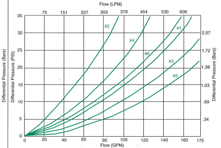
Graph 6. Effect of Viscosity on 10 Micron Media Curve 1. 265321-0000/576366-7110 at 225 SUS Curve 2. 265321-0000/576366-7110 at 600 SUS Curve 3. 267321-0000/578366-7110 at 225 SUS Curve 4. 267321-0000/578366-7110 at 600 SUS Curve 5. 269321-0000/5 & 67366-7110 at 225 SUS Curve 6. 269321-0000/5 & 67366-7110 at 600 SUS
