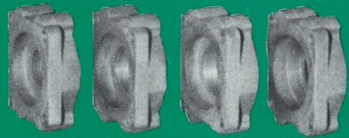
1 5/16"-12 1 5/8"-12 1 7/8"-12 2 1/2" -12
